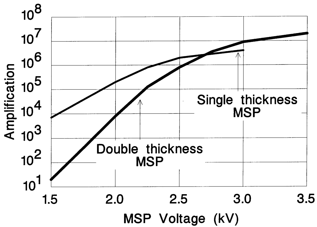
Figure 2. MSP amplification
