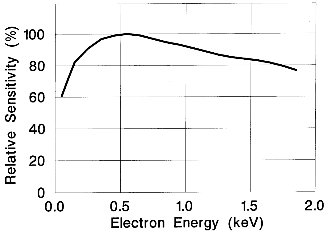
Figure 6. MSP sensitivity to electrons
