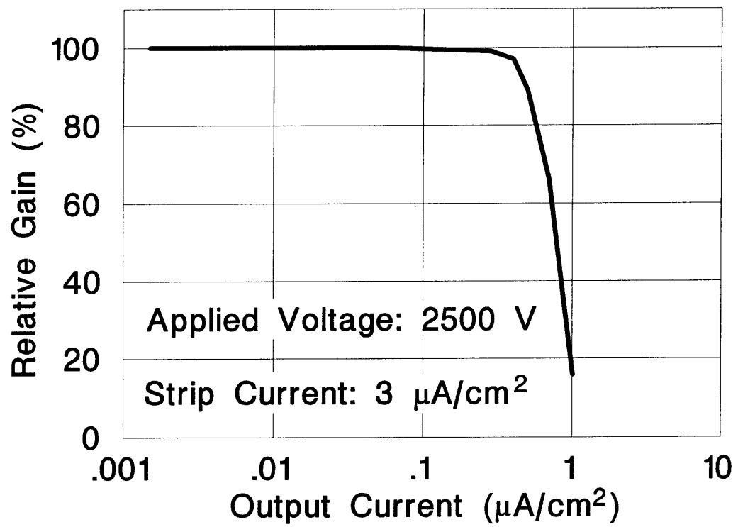
Figure 3. MSP saturation characteristics
