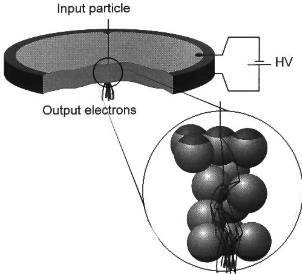
Figure 1. Schematics of MSP multiplication chain
