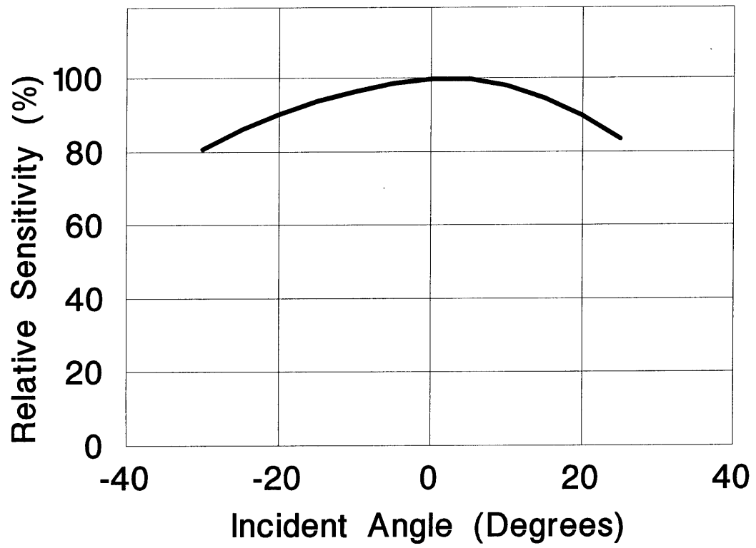
Figure 5. MSP Sensitivity vs. Incident Angle of UV photons.
