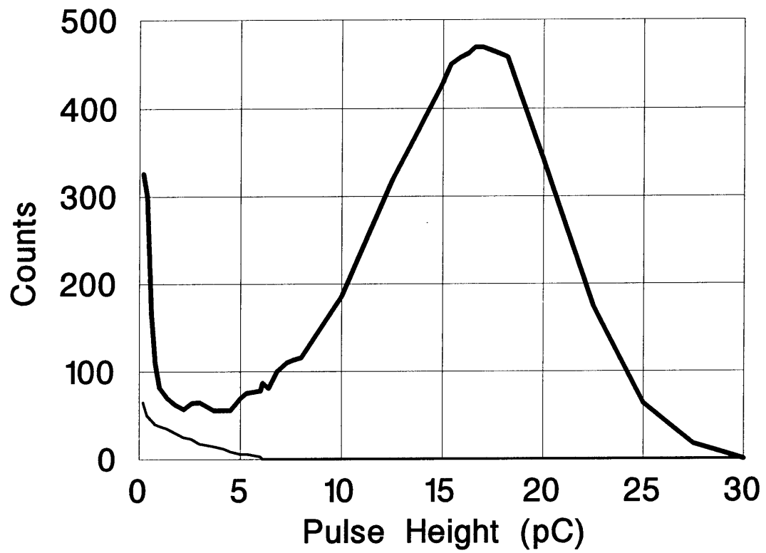
Figure 4. Double thickness MSP: Signal and noise PHD at 3.2 kV
