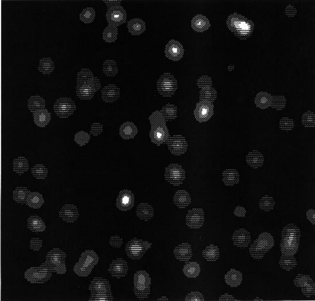
Figure 7. Single electrons hitting an MSP, as seen at the phosphor screen
