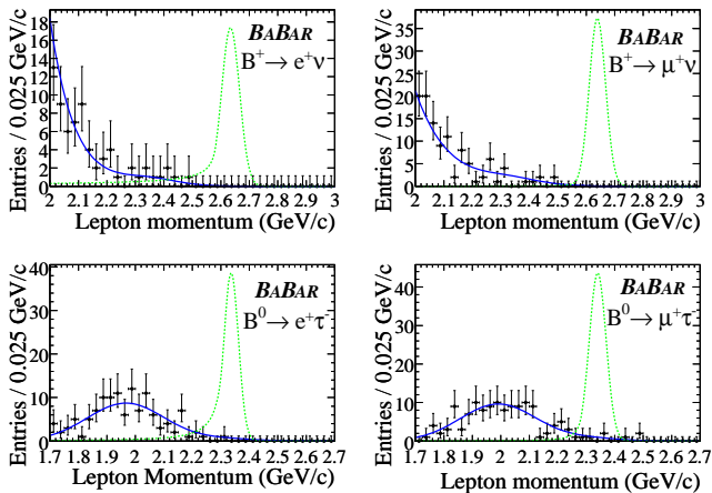
FIG. 2: The unbinned maximum likelihood fits on the lepton momentum. The dashed line, representing the signal PDF with an arbitrary scaling, indicates where the signal is expected.
