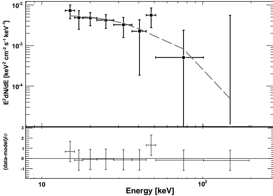
Fig. 14.— BAT spectrum of Abell 3667. The dashed line is the best fit thermal model with a temperature of 18.7_{-9.3}^{+22.6} keV.
