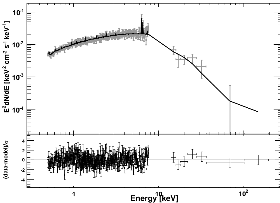
Fig. 9.— Spectrum of Abell 2256 fitted with a single temperature thermal model.
