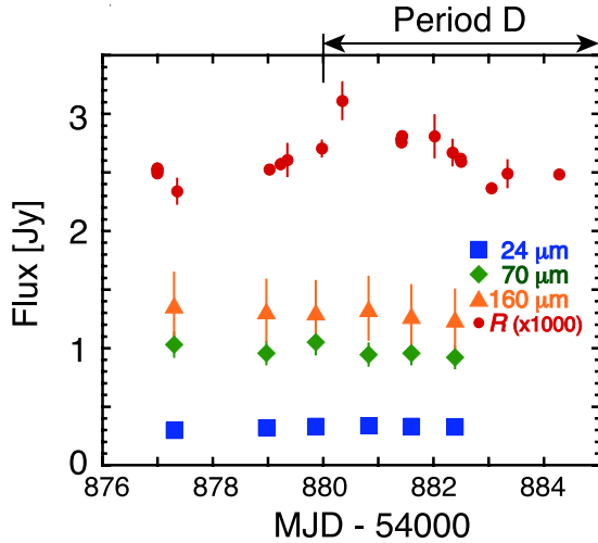
Figure 10. Light curve of 3C 279 at 24 \mu\text{m} , 70 \mu\text{m} and 160 \mu\text{m} measured by Spitzer-MIPS. The error bars correspond to 10%, 10% and 20%, respectively, for each band as mentioned in the text in Section 3.9. Optical R -band data taken by the ground-based telescopes are also plotted in red color for comparison.
