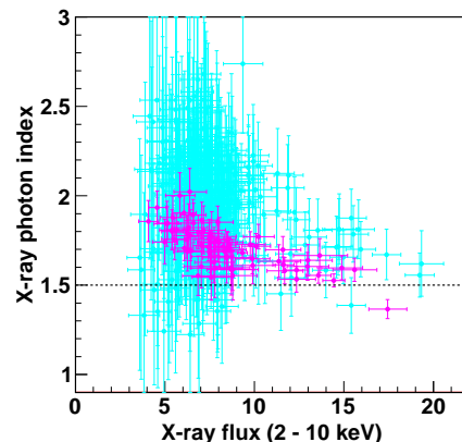
Figure 6. Scatter plot of flux vs. photon index of 3C 279 in the X-ray band with the data taken by Swift-XRT (magenta) and RXTE-PCA (cyan). The horizontal dotted line represents the photon index value of 1.5.
