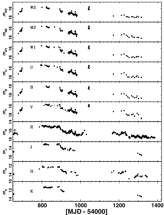
Figure 7. Light curves of all observed UV-optical-NearIR bands of 3C 279 in measured magnitude scale from 2008 August to 2010 August, including W2 ( Swift -UVOT), M2 ( Swift -UVOT), W1 ( Swift -UVOT), U ( Swift -UVOT), B ( Swift -UVOT), V (Katana, Swift -UVOT), R (Abastumani, Calar Alto, ST-7, GRT, MDM, L’Ampolla, Perkins, SLT, KVA, LT, San Pedro, St. Petersburg, Tijarafe), J (AZT-24, Kanata), H (AZT-24, LT) and K (AZT-24, Kanata) bands.
