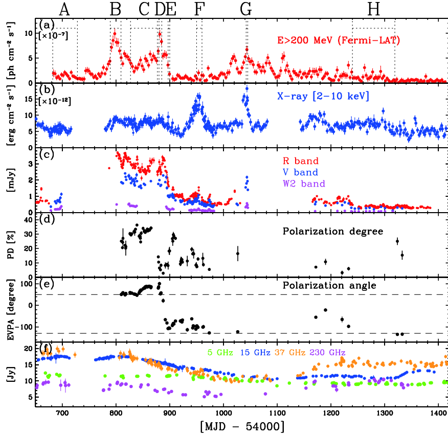
Figure 12. Multi-band light curves of 3C 279 for 2 years from 2008 August to 2010 August. (a): Gamma-ray flux above 200 MeV averaged over 3 days. (b): X-ray flux between 2 and 10 keV measured by Swift -XRT and RXTE -PCA. (c): UV-optical fluxes in R -band (red), V -band (blue) and W2 -band (magenta). (d): Polarization degree in the optical band. The horizontal dashed lines refer to the angle of 50^\circ and -130^\circ . (e): Radio fluxes in 230 GHz band (magenta), 37 GHz band (orange), 15 GHz band (blue) and 5 GHz band (green). All X-ray, UV and optical data are corrected for the Galactic absorption.
