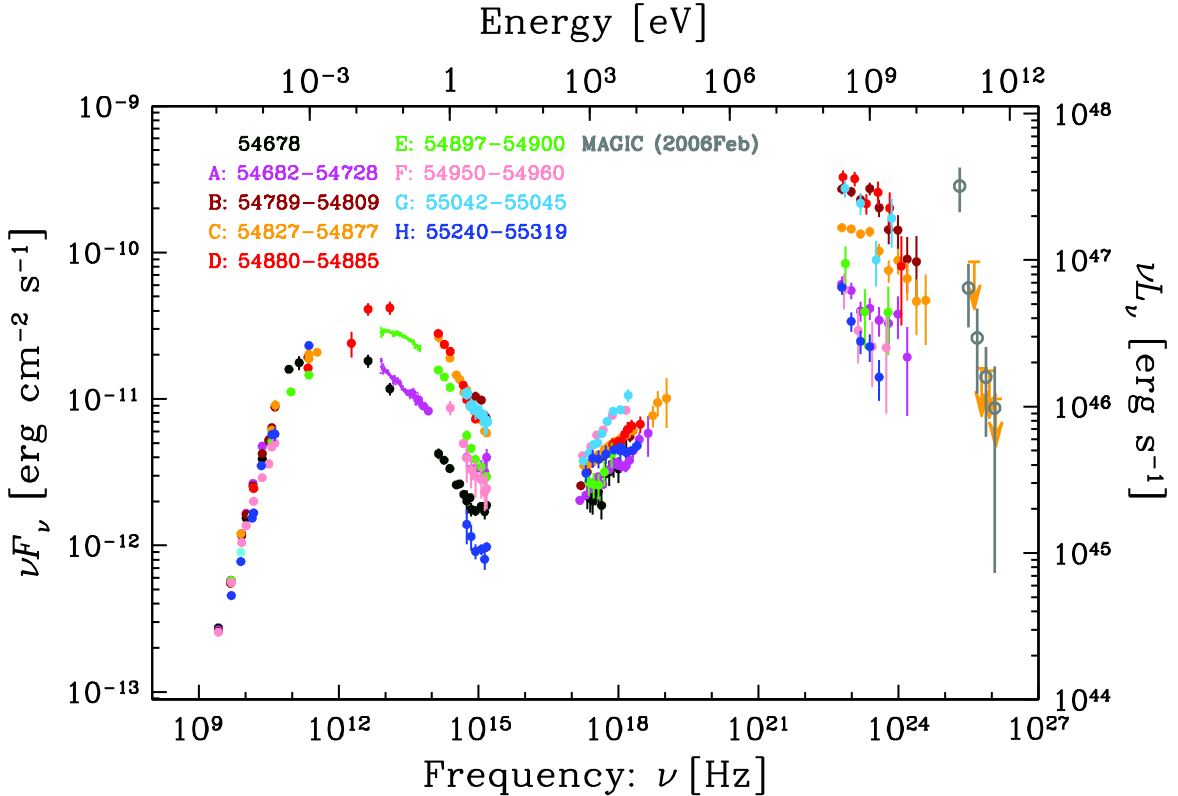
Figure 15. Time-resolved broad-band spectral energy distributions of 3C 279 measured in Period A–H (as defined in Table 1) and on 2008 July 31 (MJD 54678), covered by our observational campaigns in 2008–2010. X-ray, UV-optical-nearIR data are corrected for the Galactic absorption. 5-digit numbers in the panel indicate MJD of the periods. For comparison, the gray open circles in the very-high-energy \gamma -ray band represent measured spectral points by MAGIC in 2006 February (Albert et al. 2009).
