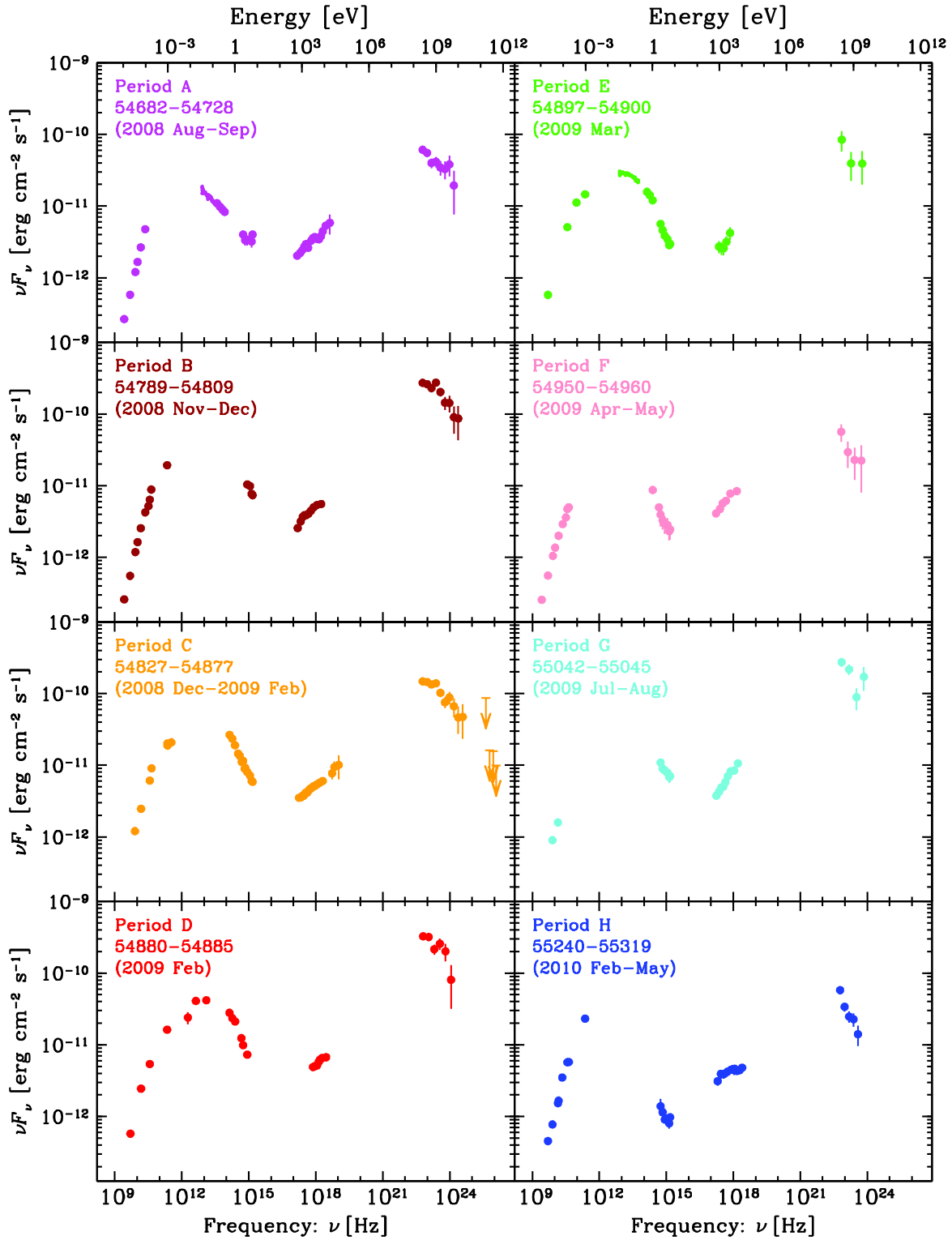
Figure 16. Time-resolved broad-band spectral energy distributions of 3C 279 in each period (A–H), covered by the campaigns. The data points are the same as ones in Fig. 15, but are plotted in a separate panel for each period. 5-digit numbers in each panel indicate MJD of the observing period of each broad-band spectrum.
