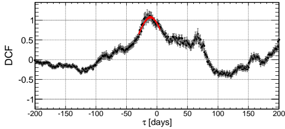
Figure 13. Discrete Correlation Function (DCF) derived for the \gamma -ray and optical R bands. Positive values of ‘ \tau ’ correspond to flux variations in the \gamma -ray band lagging flux variation in the optical band. The red curve represents a Gaussian fit to the data between -30 and 5 days. See the text for the fitting results.
