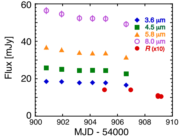
Figure 11. Light curve of 3C 279 at 3.6 \mu\text{m} , 4.5 \mu\text{m} , 5.8 \mu\text{m} and 8.0 \mu\text{m} measured by Spitzer-IRAC. The error bars correspond to 3% for all IRAC bands as mentioned in the text in Section 3.9. Optical R -band data taken by the ground-based telescopes are also plotted in red color for comparison.
