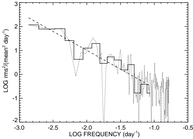
Figure 2. Power Density Spectrum of 3C 279 for the 3-day binned \gamma -ray light curve. The white noise level has been subtracted. The solid line histogram describes the PDS averaged in logarithmic frequency bins while the dotted curve describes the raw PDS before binning. The dashed line represents a linear fit to the binned PDS.
