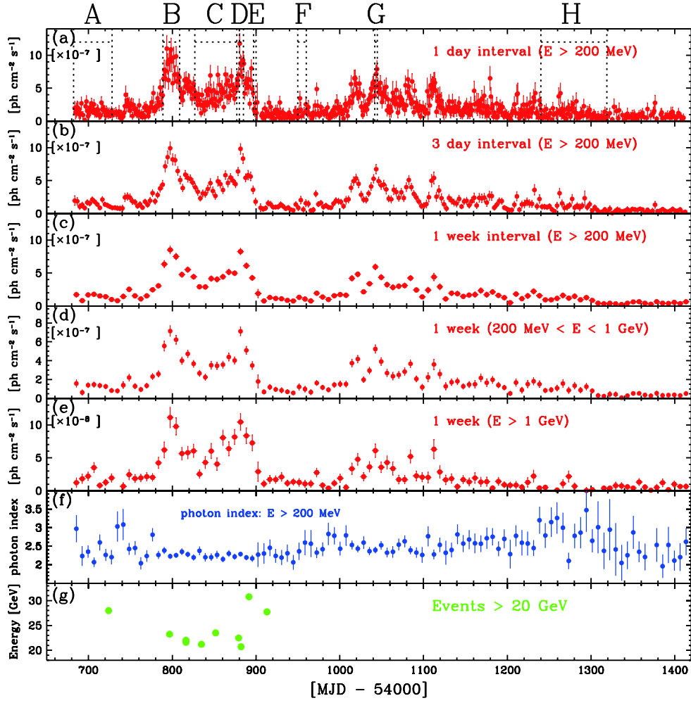
Figure 1. Gamma-ray light curves of 3C 279 during the first two years of the Fermi -LAT observations from 2008 August to 2010 August, plotted in; (a) 1-day intervals at energies above 200 MeV, (b) 3-day intervals at energies above 200 MeV, (c) 1-week intervals at energies above 200 MeV, (d) 1-week intervals at energies between 200 MeV and 1 GeV, (e) 1-week intervals at energies above 1 GeV. The panel-(f) shows the history of the photon index at energies above 200 MeV in 1 week intervals, while the panel-(g) shows arrival time distribution of > 20 GeV events associated with 3C 279. The vertical axis of the panel-(g) represents the estimated energy of events. The highest energy photon corresponds to 30.8 GeV at MJD 54891. The dotted lines and capital letters represent time intervals where \gamma -ray spectra are extracted (see also Table 1).
