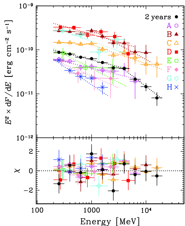
Figure 4. Gamma-ray spectral energy distributions of 3C 279 of each period as defined in the text or Table 1. 2-year averaged [black: filled circles], Period A (magenta: open circles), Period B (brown: filled triangles), Period C (orange: open triangles), Period D (red: filled squares), Period E (green: open squares), Period F (pink: filled diamonds), Period G (cyan: open diamonds) and Period H (blue: crosses). The vertical bars indicate 1\sigma statistical errors while the horizontal bars indicate energy ranges of each bin. The best-fit spectral models are plotted as dotted lines for each period and their parameters are summarized in Table 1. We use the broken power law model for the spectra of 2-year, Period B and Period C because significant improvements in the spectral fits can be seen compared to the simple power law model (see Table 1) while the simple power law model is used for other periods. The lower panel shows the residuals, plotted as \chi \equiv (\text{data} - \text{model})/\text{data error} from the best-fit models. A ‘dip’ feature at \sim 1\text{--}2 GeV in the spectrum of Period G (the 3rd point in cyan) is a \leq 2\sigma effect from the best-fit model, thus, not statistically significant.
