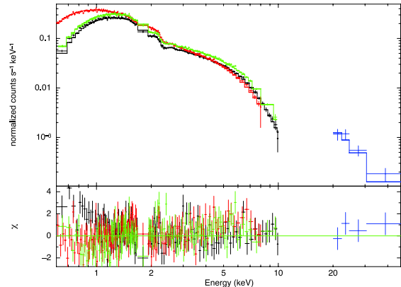
Figure 5. Count spectra of 3C 279 measured by Suzaku XIS0 (black), XIS1 (red), XIS3 (green) and HXD/PIN (blue). The model plotted with the data is a broken power law obtained by a fitting these three XISs and HXD/PIN data. The lower panel shows the residuals for this broken power law model.
