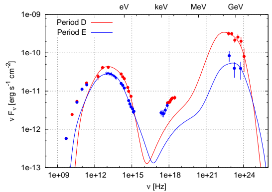
Figure 17. Emission models D1 (red line) and E1 (blue line) fitted to the spectral states at Periods D and E, respectively. Periods D and E correspond to the first 5 days and the last 3 days of the \gamma -ray flaring event accompanied by an optical polarization change, respectively. Those models adopt our ‘propagation scenario’, where external radiation is dominated by infrared dust emission. We assume the X-ray emission is not related to the flaring component, and consider the X-ray fluxes as only upper limits to the SSC and the ERC components during the flaring event. See the text in Section 5 and 5.1 for details of the models and Table 5 for model parameters.
