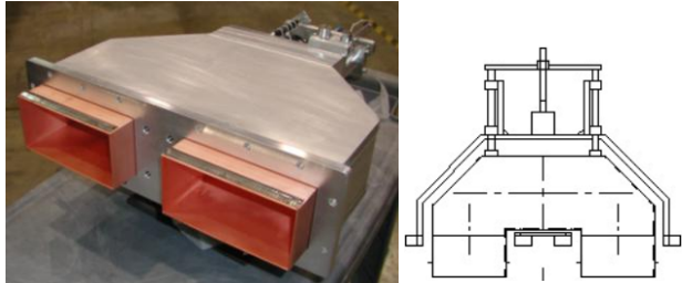
Figure 4: Photograph of a U-bend phase shifter with fingerstock to contact mating waveguide and drawing showing interior construction and pressure feed-throughs.
