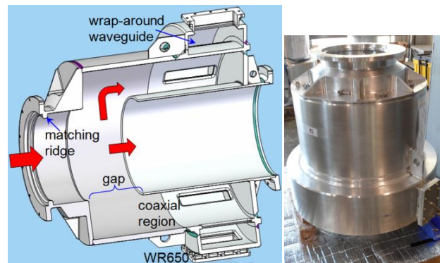
Figure 1: Descriptive design illustration and photograph of a 3-dB prototype Coaxial Tap-Off (CTO).
