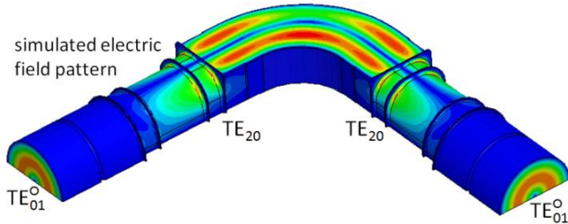
Figure 2: Half geometry of the circular TE 01 mode bend design with electric field patterns illustrating mode conversion in the interior.
