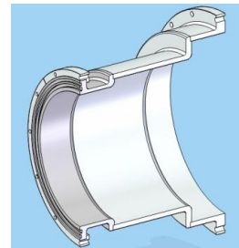
Figure 6: WC1375–WC1890 step taper for KCS.
