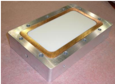
Figure 5: Photograph of the ceramic block window.
