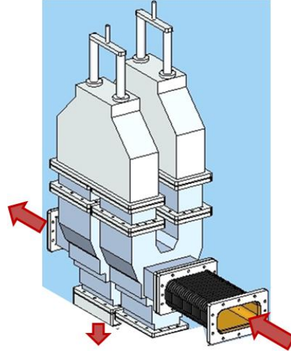
Figure 3: Variable Power Divider (VPD), composed of folded magic Ts and U-bend phase shifters.
