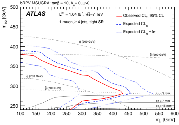
FIG. 9: Observed and expected 95% CL exclusion limits, as well as the \pm 1\sigma variation on the expected limit, for the bilinear R-parity violation model in MSUGRA parameter space using the 4JT selection in the muon channel. The region with LSP lifetimes c\tau > 15 mm is not shown.
