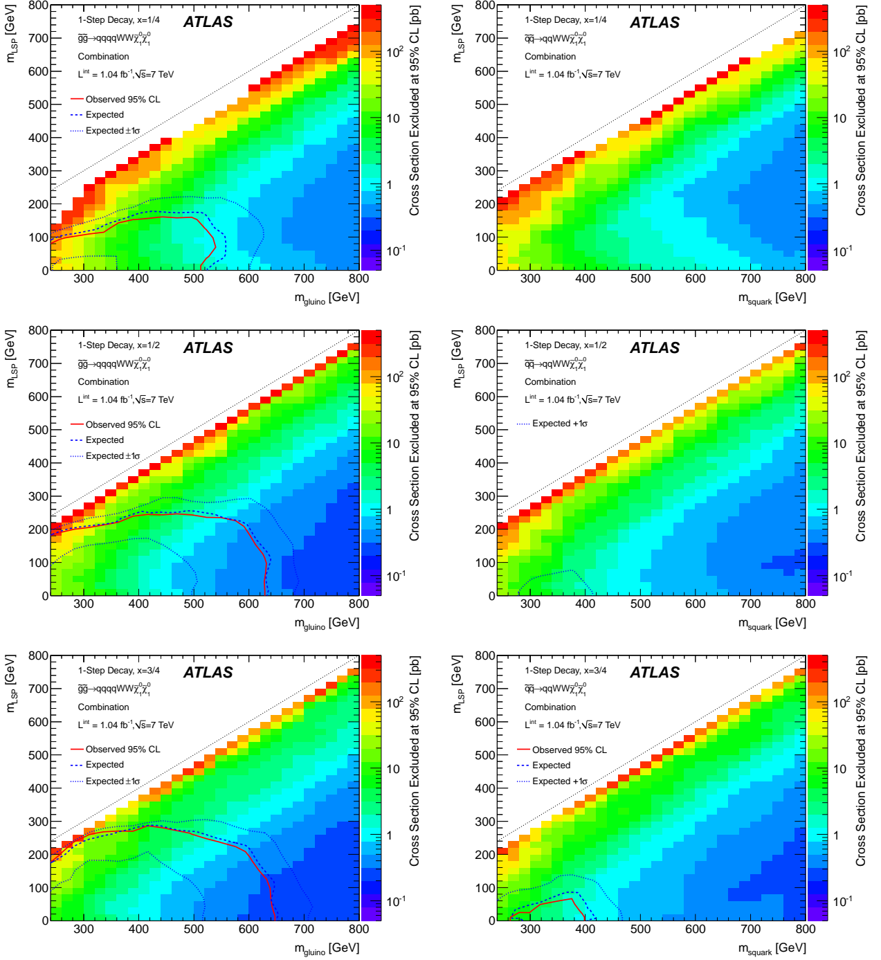
FIG. 8: Excluded cross-sections at 95% confidence level for the simplified models. The left column shows the results for the gluino models, the right column shows the results for the squark models. The top row plots represent the case x = 1/4 , the middle row x = 1/2 , and the bottom row x = 3/4 . The color coding (right axis) represents the model-independent cross-section limit. Full lines indicate the observed exclusion regions in the shown plane assuming production cross-sections as calculated with PROSPINO for the MSSM, and a 100% branching fraction into the assumed decay modes. The dashed line shows the corresponding median expected limit and the dotted lines show the \pm 1\sigma variation of the expected limit.
