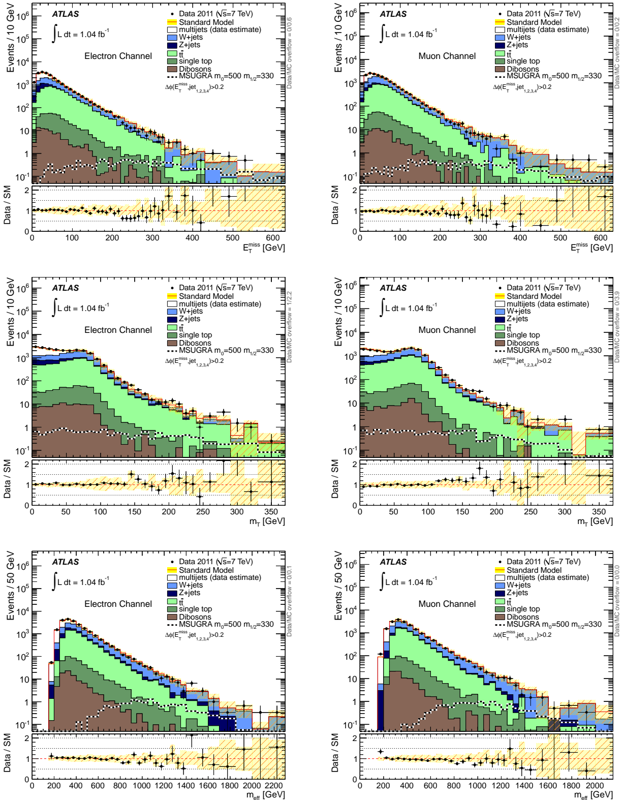
FIG. 2: Distributions after requiring one electron with p_T > 25 GeV or one muon with p_T > 20 GeV, and at least four jets with p_T > 60, 25, 25, 25 GeV and \Delta\phi(\text{jet}_i, \vec{E}_T^{\text{miss}}) > 0.2 . The top row shows the missing transverse momentum, the middle row shows the transverse mass, and the bottom row displays the effective mass. The electron channel is shown in the left column, the muon channel is shown in the right column. The “Data/SM” plots show the ratio between data and the summed standard model expectation. In these plots, the standard model expectation is derived from Monte Carlo simulations only, normalized to the theoretical cross sections. The uncertainty band on the standard model expectation combines the MC statistical uncertainty and systematic uncertainties on the jet energy scale and resolution, the lepton resolution and identification efficiencies, pile-up and luminosity. For illustration, the expected signal distributions of the MSUGRA/CMSSM model point m_0 = 500 GeV, m_{1/2} = 330 GeV are also shown.
