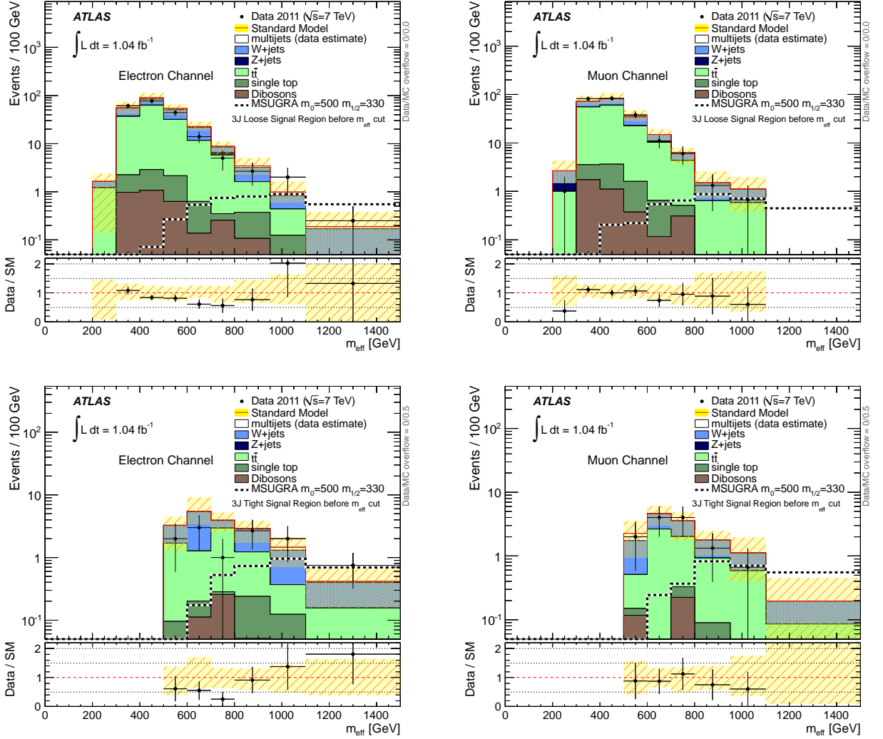
FIG. 5: Distributions of the effective mass for events in the 3-jet signal regions 3JL (top) and 3JT (bottom) for the electron channel (left) and the muon channel (right), after application of the final selection criteria described in Section VII A, except for the cut on m_{\text{eff}} itself. The “Data/SM” plots show the ratio between data and the summed standard model expectation. The uncertainty band on the standard model expectation combines the MC statistical uncertainty and systematic uncertainties on the jet energy scale and resolution, the lepton resolution and identification efficiencies, pile-up and luminosity. For illustration, the expected signal distributions of the MSUGRA/CMSSM model point m_0 = 500 GeV, m_{1/2} = 330 GeV are also shown.
