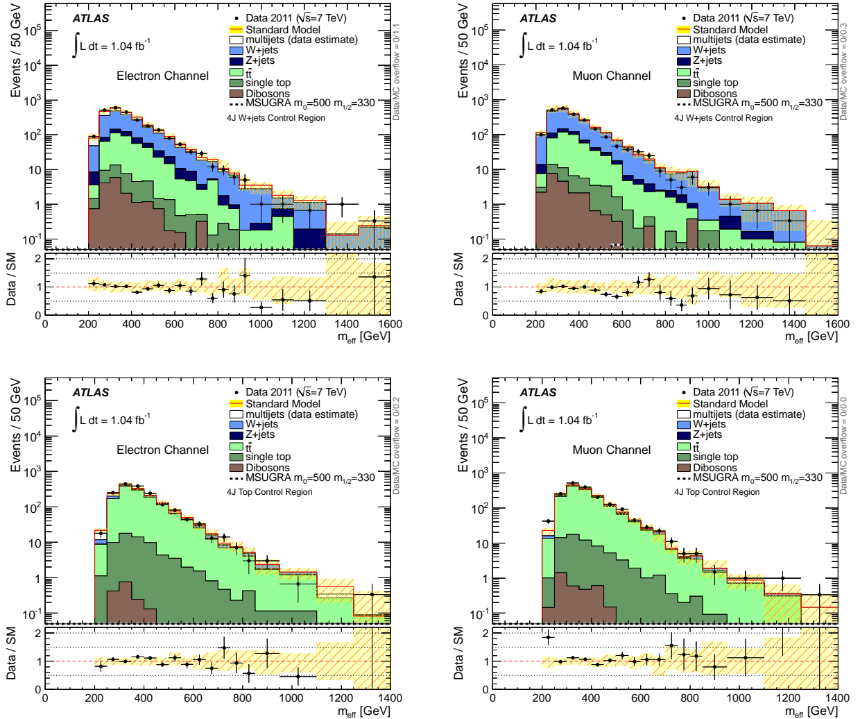
FIG. 4: Distributions for events in the lepton plus four jets control regions for the electron channel (left column) and muon channel (right column). Top row: effective mass in the W +jets control region. Bottom row: effective mass in the top control region. The “Data/SM” plots show the ratio between data and the summed standard model expectation. The uncertainty band on the standard model expectation combines the MC statistical uncertainty and systematic uncertainties on the jet energy scale and resolution, b -tagging, the lepton resolution and identification efficiencies, pile-up and luminosity.
