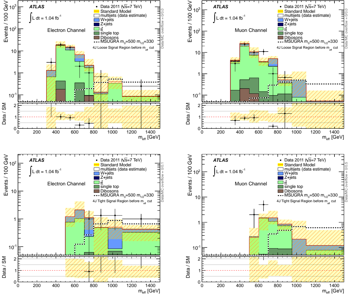
FIG. 6: Distributions of the effective mass for events in the 4-jet signal regions 4JL (top) and 4JT (bottom) for the electron channel (left) and the muon channel (right), after application of the final selection criteria described in Section VII A, except for the cut on m_{\text{eff}} itself. The “Data/SM” plots show the ratio between data and the summed standard model expectation. The uncertainty band on the standard model expectation combines the MC statistical uncertainty and systematic uncertainties on the jet energy scale and resolution, the lepton resolution and identification and luminosity. For illustration, the expected signal distributions of the MSUGRA/CMSSM model point m_0 = 500 GeV, m_{1/2} = 330 GeV are also shown.
