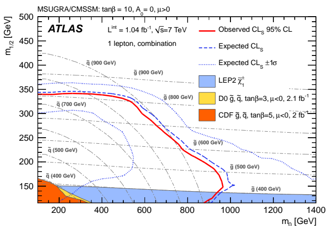
FIG. 7: Observed and expected 95% CL exclusion limits, as well as the \pm 1\sigma variation on the median expected limit, in the combined electron and muon channels. The plots also show the published limits from CDF [60], D0 [61], and the results from the LEP experiments [62].
