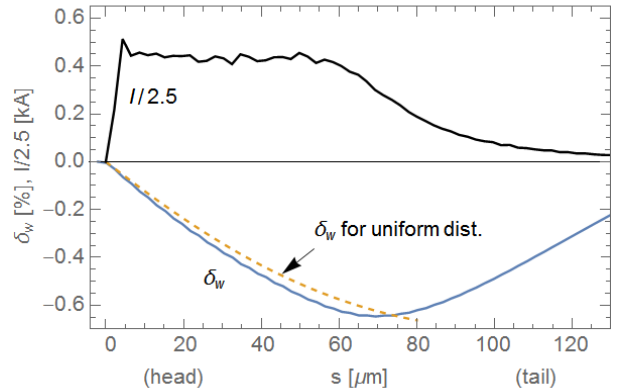
Figure 3: Relative induced voltage for realistic bunch distributions (blue), for Q = 100 pC (top), 300 pC (bottom). Dashes gives result for uniform distributions. Current shape given in black, with head to the left. Bunch shapes were obtained by L. Wang.
