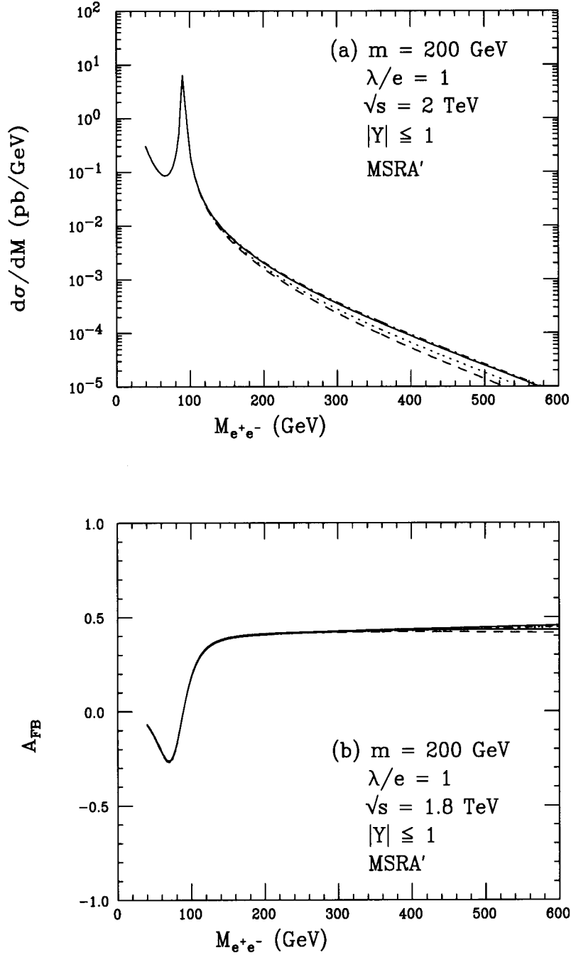
Figure 4: (a) The lepton pair invariant mass distribution and (b) forward-backward asymmetry in Drell-Yan production for the SM (solid curve) and with 200 GeV scalar leptoquark exchange, assuming \tilde{\lambda} = 1 , with left-(right-)handed couplings to u-quarks, corresponding to the dashed (dotted) curve, and left-(right-)handed couplings to d-quarks (dash-dotted curve for both cases).
