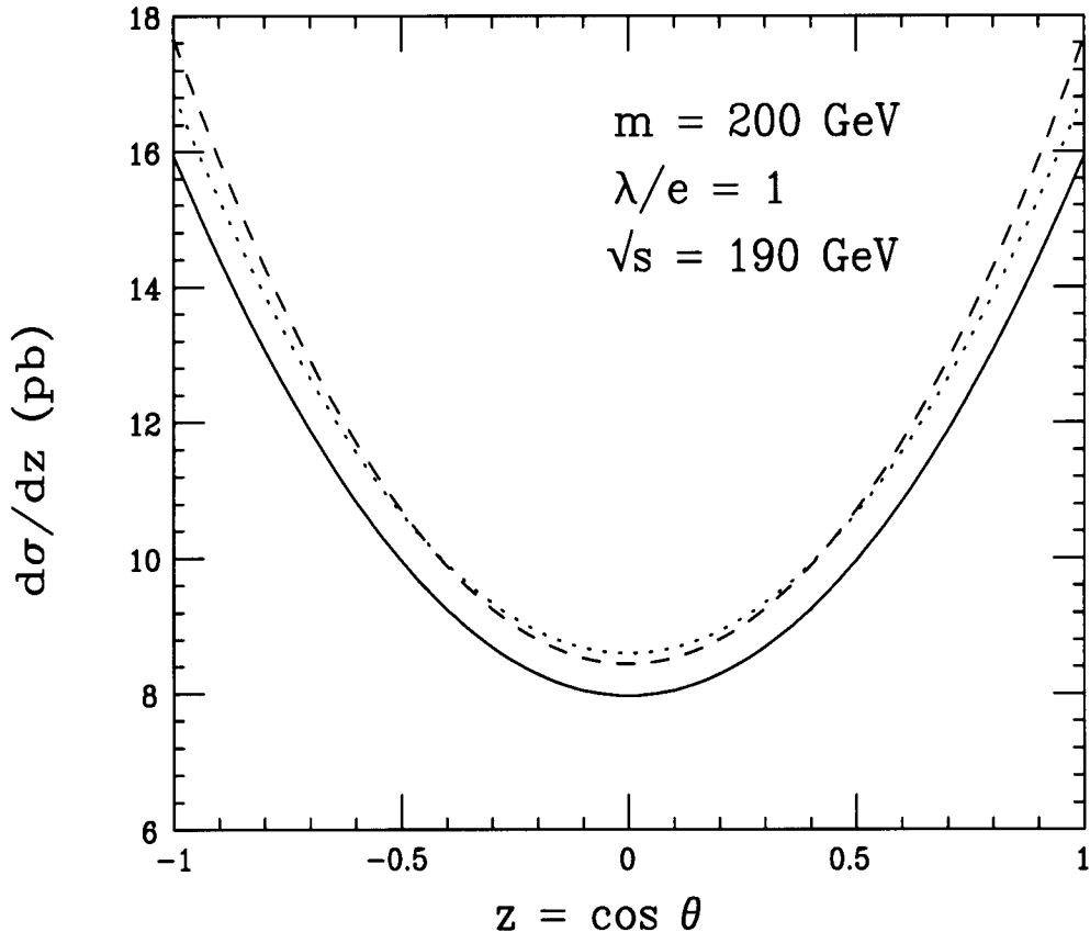
Figure 8: Symmetrized angular distribution of q\bar{q} final states in e^+e^- annihilation at 190 GeV with z = \cos \theta . The solid curve is for the SM while the dotted(dashed) curve includes the contribution of a 200 GeV scalar(vector) leptoquark coupling to d_L with \tilde{\lambda} = 1 .
