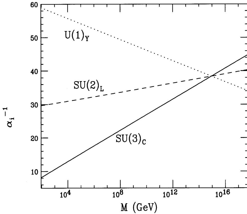
Figure 10: Two-loop RGE evolution of the model with the SM particle content together with a pair of \tilde{R}_{2L} type leptoquarks and an additional Higgs doublet.
