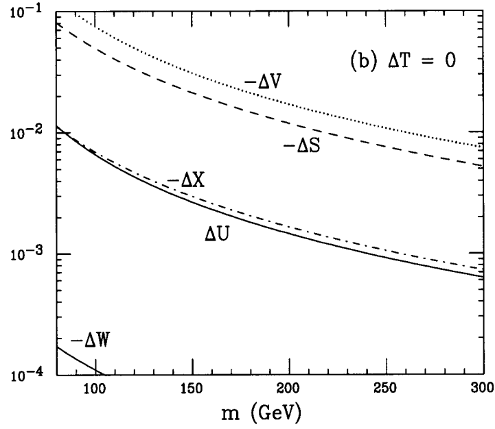
Figure 7: Shifts in the oblique parameters as functions of the leptoquark mass for the (a) \tilde{R}_{2L} and (b) R_{2L} or R_{2R} cases.
