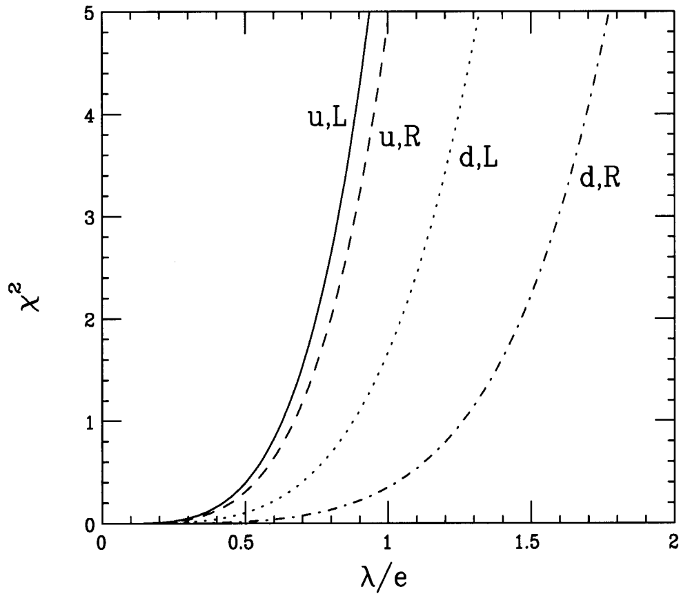
Figure 6: \chi^2 fits to Drell-Yan production including the effects of a 200 GeV scalar leptiquark for each type of leptiquark coupling as labeled. The 95% C.L. constraints are obtained when \chi^2 = 3.842 .
