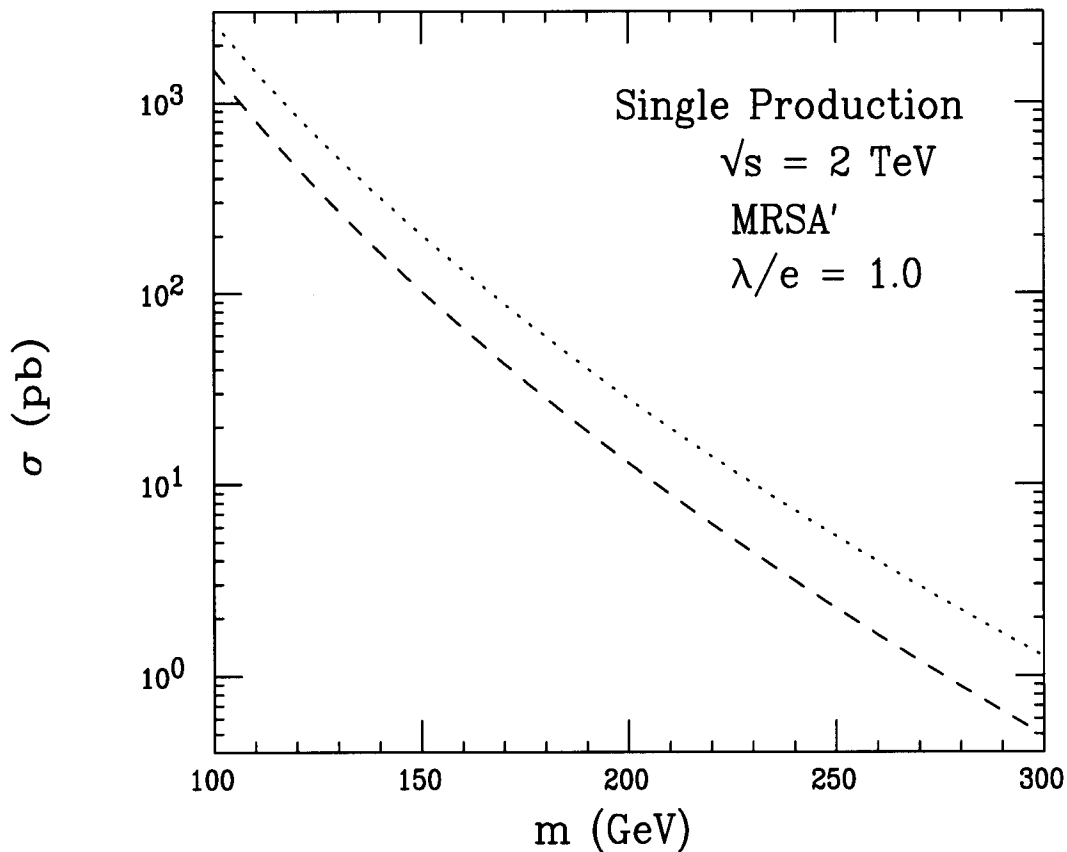
Figure 3: Single production cross sections at the Tevatron for scalar leptoquarks as a function of mass from gu(\bar{u}) and gd(\bar{d}) fusion, corresponding to the dotted and dashed curves, respectively. Here, \lambda/e = 1 , and the K-factor has been omitted.
