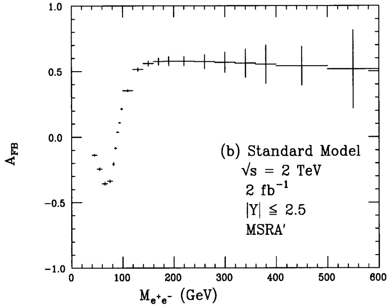
Figure 5: Bin integrated lepton pair (a) invariant mass distribution and (b) forward-backward asymmetry for Drell-Yan production in the SM at the Main Injector. The vertical lines correspond to the expected statistical error in each bin.
