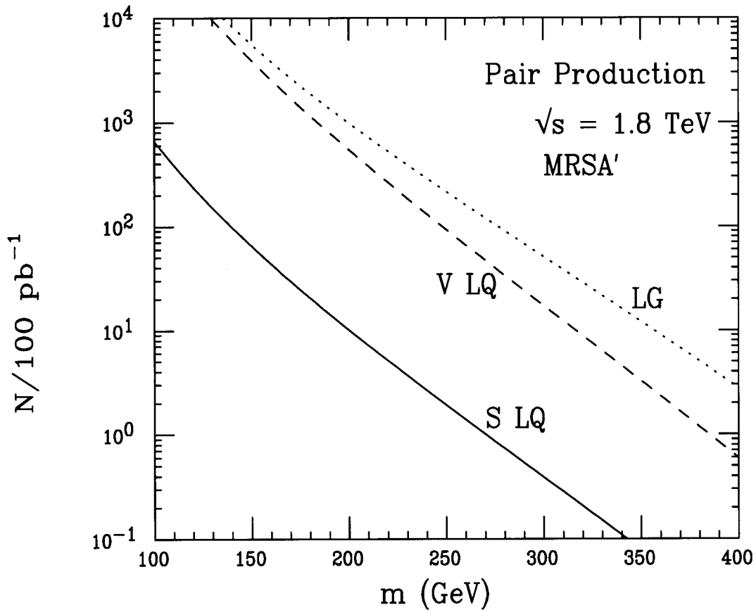
Figure 1: Pair production cross sections at the Tevatron for scalar and vector leptoquarks, as well as leptogluons, corresponding to the solid, dashed, and dotted curves, respectively. Here, the gg and q\bar{q} contributions are summed.
