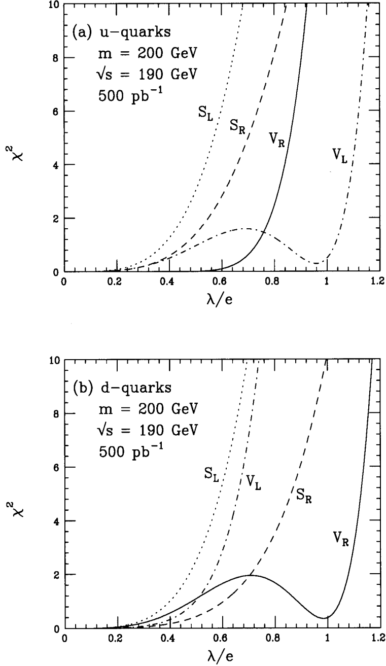
Figure 9: \chi^2 fits to the SM angular distribution for e^+e^- \rightarrow q\bar{q} at 190 GeV including the effects of a 200 GeV leptoquark coupling to (a) u- or (b) d-quarks. In both cases the dotted(dashed) curve corresponds to a scalar leptoquark with a left(right)-handed coupling while the dash-dotted(solid) curve corresponds to the vector leptoquark case with left(right)-handed couplings. The 95% CL limits are obtained when \chi^2 = 3.842 .
