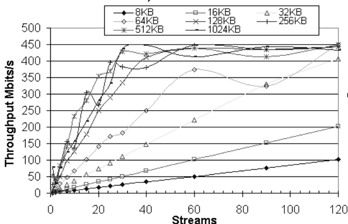
Figure 6: Ten second iperf TCP throughputs from SLAC to ANL as a function of TCP window size and streams.
