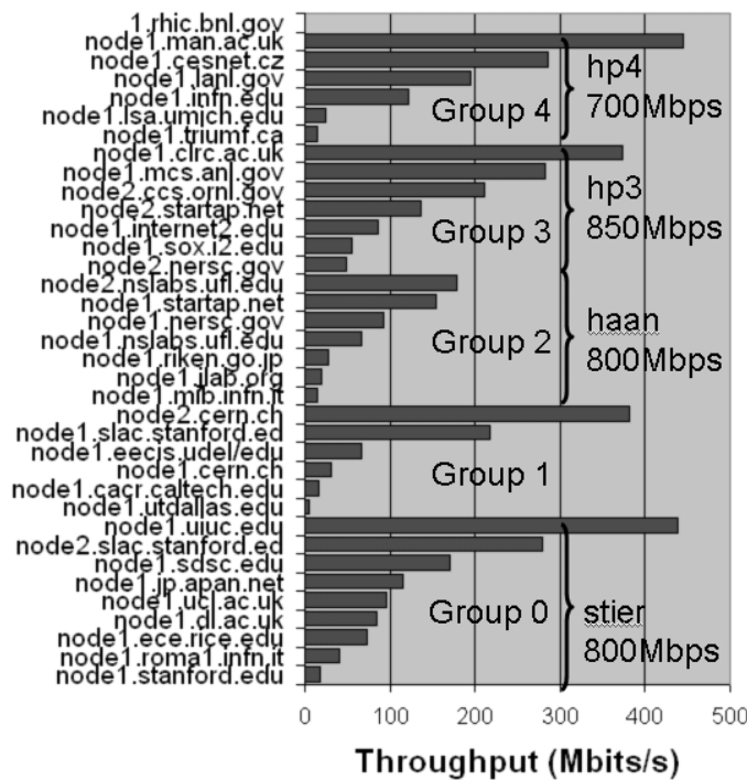
Figure 8: Iperf TCP sequential throughputs for remote host groups measured from keeshond at iGrid2002. The flood throughputs measured from stier are also shown, together with which group was assigned to which monitoring host.
