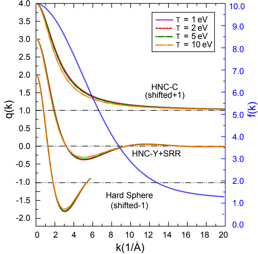
Figure 23. Three screening functions q(k) are shown for temperatures ranging from 1 eV to 10 eV along with the atomic form factor f(k) . While HNC-Y+SRR and hard sphere models agree well with the data, models that only include screening provide a poor match with the data.
