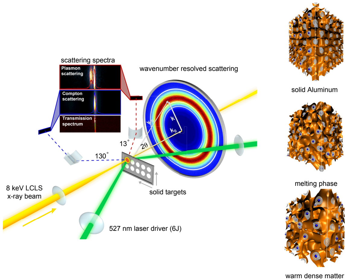
Figure 19. (Top) A schematic of experimental setup for compressed matter studies at MEC is shown. The LCLS x-ray beam is focused into the dense laser-compressed aluminium target. The 13^\circ forward x-ray scattering spectrum shows inelastic plasmon scattering together with the elastic scattering feature at the incident x-ray energy. The 130^\circ backscattering shows no scattering feature in this energy range validating the identification of the plasmon. A CSPAD area detector observes the total wavenumber-resolved x-ray scattered intensity indicating the transition from Debye-Scherrer diffraction rings (white) to an intense ion-ion correlation scattering feature (red). (Bottom) DFT-MD simulations of the formation of WDM indicate that the ions (blue) abandon their lattice positions. Whilst core electrons (grey) remain mostly unchanged the delocalized conduction electrons (represented by orange iso-surfaces) are disturbed from the very regular structure in the lattice.
