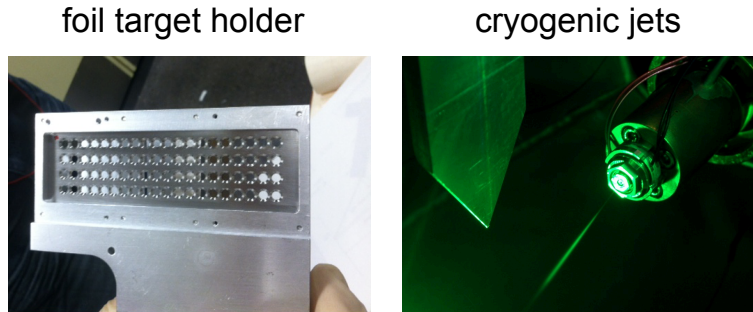
Figure 7. (Left) The target holder is shown for solid target experiments. The long pulse lasers heat the foil that is mounted in one opening in a single dynamic compression experiment. Subsequent experiments use a new foil target in the next opening. (Right) An example of a continuous cryogenic jet is shown. These targets allow experiments at high repetition rates. Pump-probe studies using LCLS combined with the short pulse laser have been demonstrated at 5 Hz.
