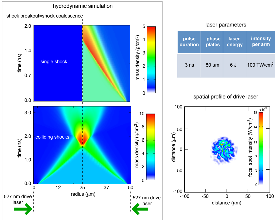
Figure 14. (Left) Radiation-hydrodynamic design of single shock wave experiments and counter-propagating shocks driven by two MEC nanosecond lasers with the same pulse shape. (Right, bottom) The focal spot diameter is obtained from phase plate characterization data.
