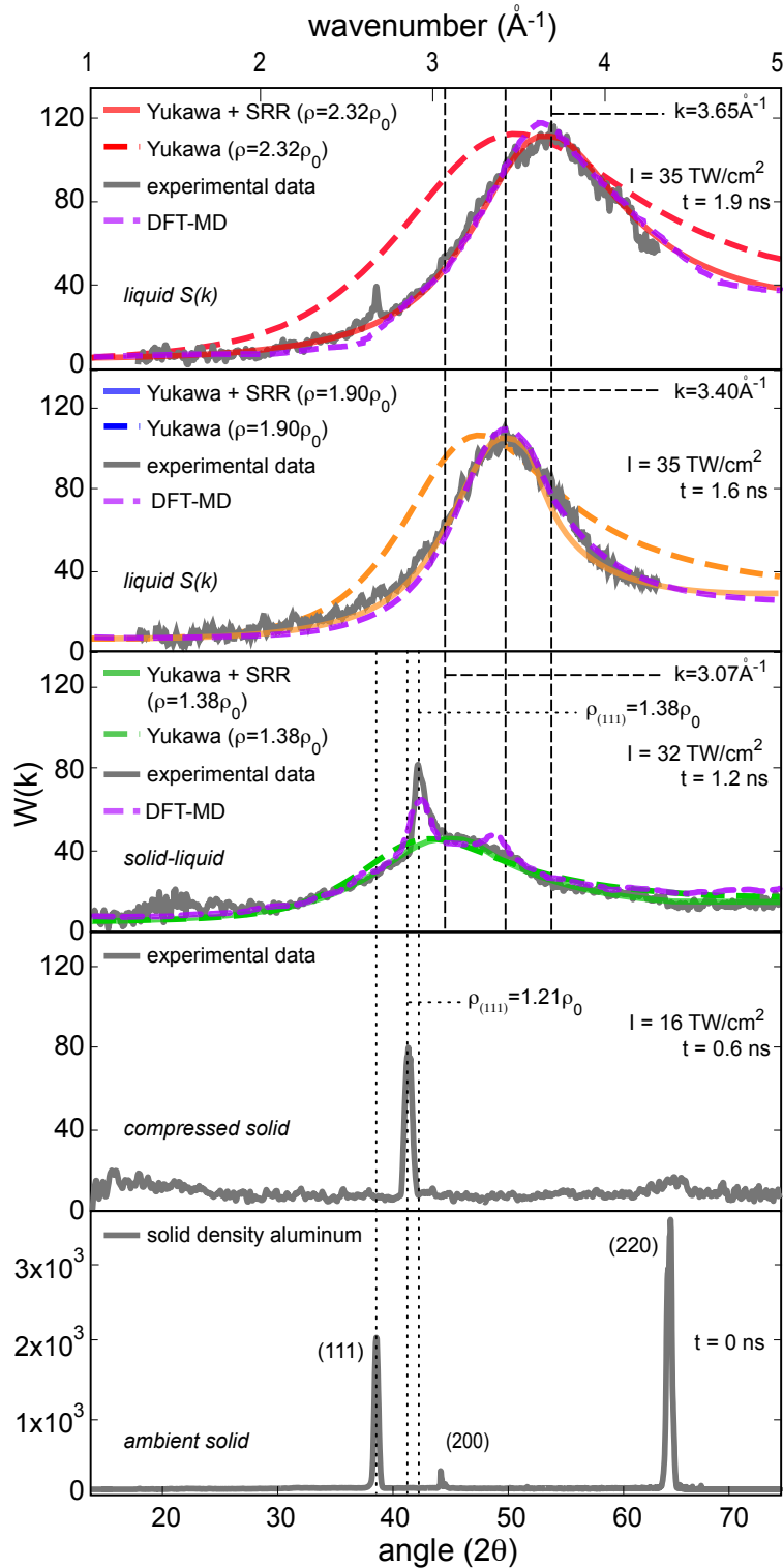
Figure 22. X-ray scattering data W(k) are shown as function of scattering angle. (Bottom) Bragg peaks from Debye-Scherrer rings are shown at t = 0 ns. (2 nd from bottom) Data from compressed solid aluminium show a shift of the (111) Bragg peak by 3^\circ and compression of 1.21 \rho_0 . (Middle) Appearance of a broad ion-ion correlation peak is observed together with a Bragg peak shifted further to larger angles. (2 nd from top) At higher compression, aluminium melts, Bragg peaks disappear, and the ion-ion correlation peak shifts to 50^\circ . (Top) The angle of the correlation peak increases further to 56^\circ when higher densities are reached after coalescence. The data (black curves) show excellent agreement with DFT-MD simulations (top
