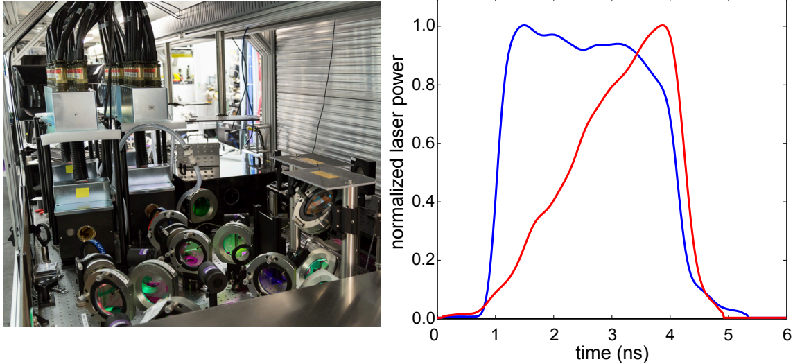
Figure 8. (Left) Picture of MEC Nd:glass laser system showing the 25 mm rod amplifiers. A laser pulse shaping system delivers about 4.5 J in 3 ns per beam on target at 527 nm. (Right) Examples of laser pulse shapes are shown for shock (blue) and ramp wave (red) compression experiments.
