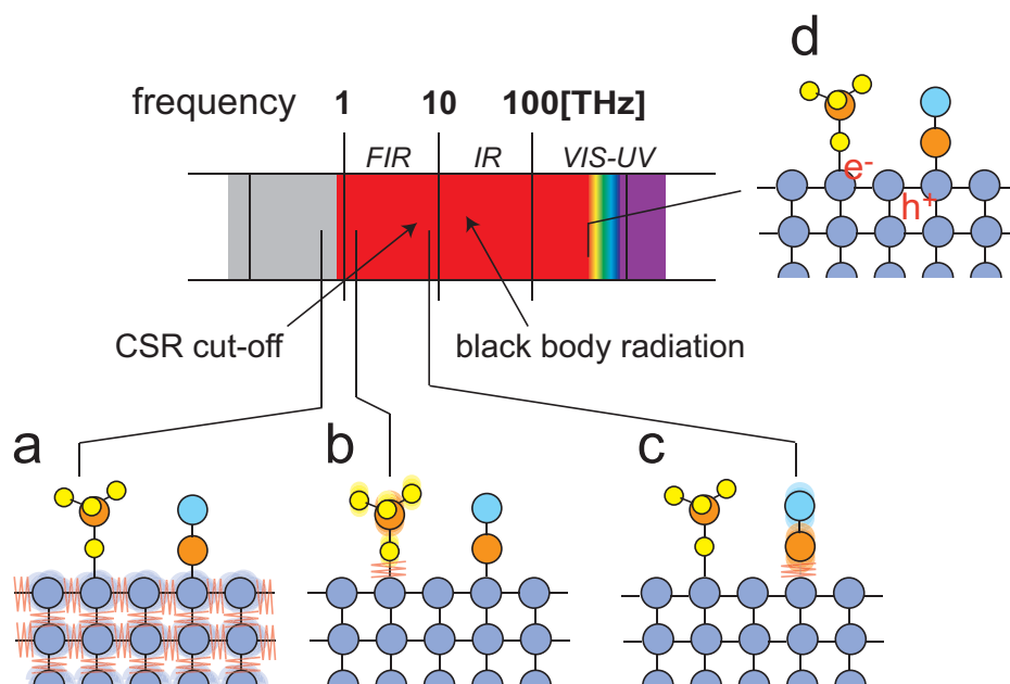
Figure 3: Excitation at surfaces. a) lattice vibration of the substrate (photon), b) frustrated vibrational motion of the physisorbed (weakly adsorbed) species, c) frustrated vibrational motion of the chemisorbed (strongly adsorbed) species, d) Visible ultrafast laser pulses predominantly produce electron-hole pairs in the substrate. The arrows indicate the maximum frequency of black body radiation at room temperature and typical coherent synchrotron radiation cut-off.
