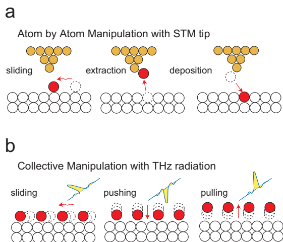
Figure 4: a) Atom by atom manipulation with a STM tip [8]. b) Collective manipulation with strong photon field with half cycle electric field pulse in different directions to the surface.
