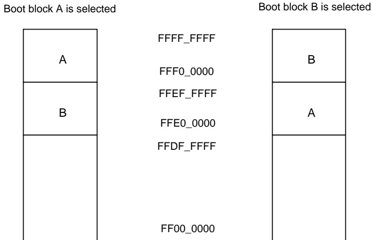
Figure 3-1 Boot Flash Bank
