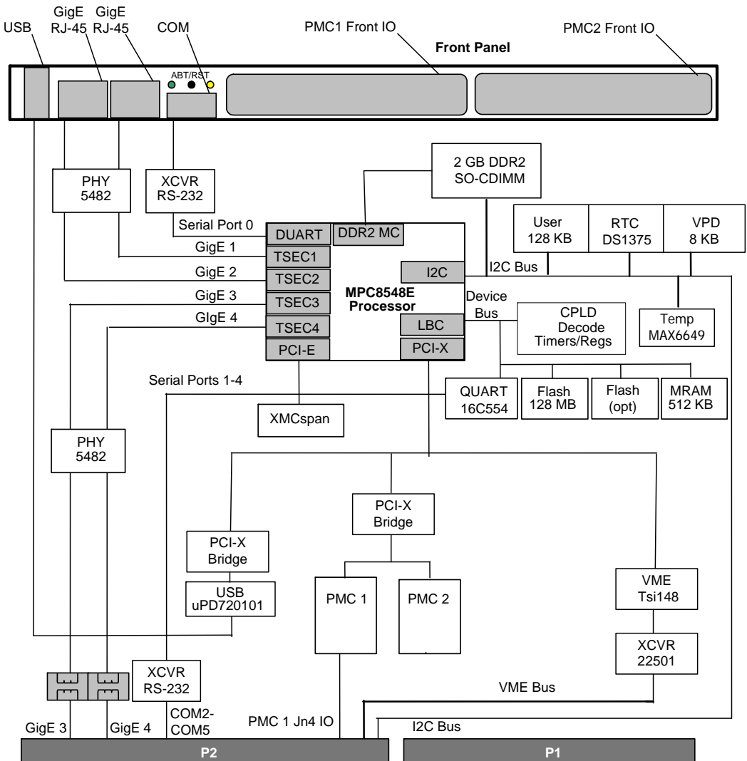
Figure 1-1 Block Diagram
