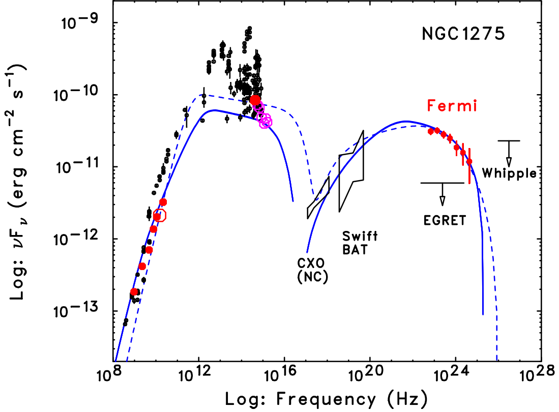
Fig. 7.— Overall SED of NGC 1275 constructed with multiband data, using radio (RATAN-600 in filled red circle; this work), radio core (MOJAVE in open red circle; this work), optical (MITSuME in red; this work), optical/UV (Swift/UVOT in open magenta circle; this work), radio to X-ray (NED), non-thermal X-ray nuclear emission (Balmaverde et al. 2006), hard X-ray (Swift/BAT; reconstructed from Ajello et al. 2009), EGRET upper limit (Reimer et al. 2003), Whipple upper limit (Perkins et al. 2006), and Fermi (this work). The RATAN, MOVAVE and MITSuME data are contemporaneous with the Fermi data. Swift UVOT data come from most recent archival observation in December 2007. The SED is fitted with a one-zone synchrotron/SSC model (blue dashed curve) and a decelerating flow model (Georganopoulos and Kazanas 2003b; blue solid curves). See text for parameters.
