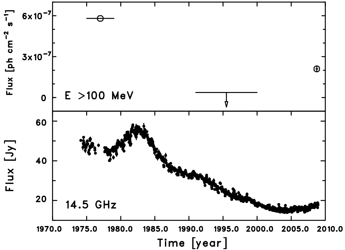
Fig. 5.— upper ; Historical gamma-ray activity of 3C 84 measured above 100 MeV. COS-B flux in this energy range was estimated by assuming a differential spectral index of \Gamma = 2.0 . lower ; A long-term radio light curve of 3C 84 taken with the UMRAO at 14.5 GHz between February 1974 and December 2008. Data are binned with daily averages. The radio light curve is in a rising state during the Fermi observations.
