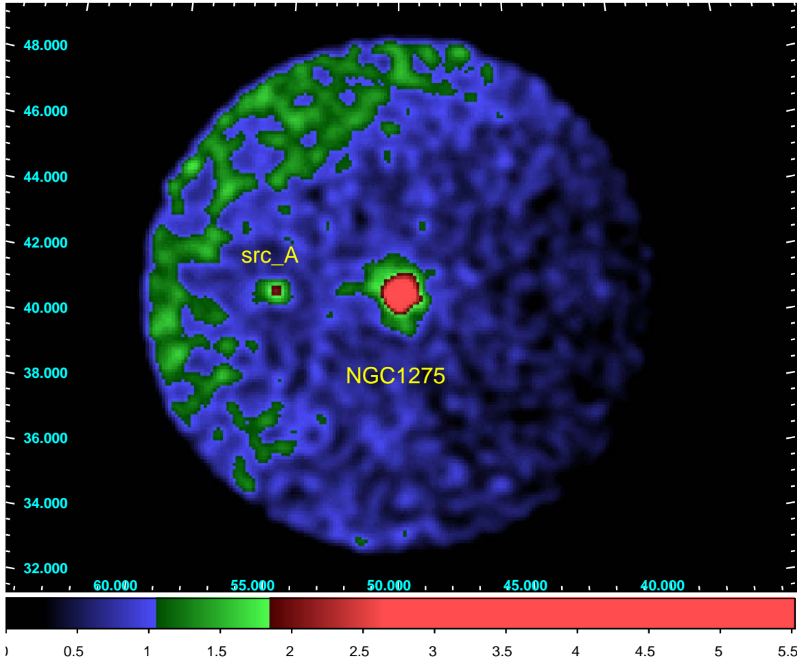
Fig. 1.— A \gamma -ray sky map obtained with Fermi at E > 200 MeV, centered on NGC 1275 (image radius r = 8^\circ , which is the value used throughout this paper). Sky survey data between August 4 and December 5 are accumulated. Full details are given in the text.
