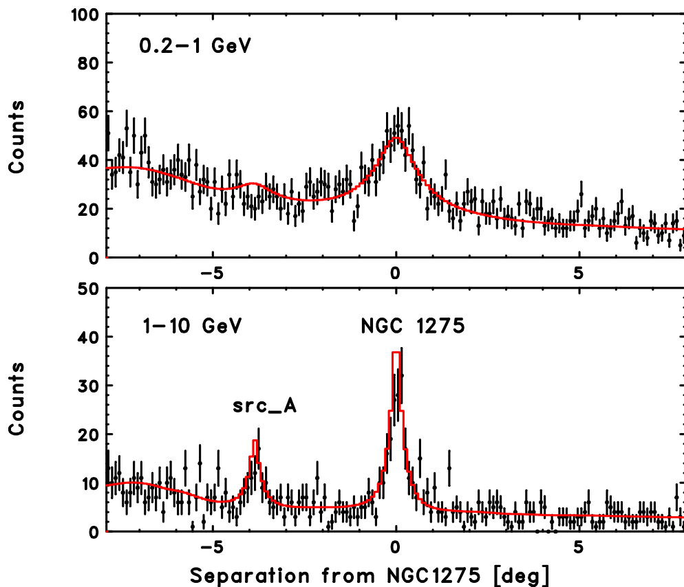
Fig. 2.— Comparison between data (black points) and GTLIKE model (red solid line) in low (0.2–1 GeV: upper ) and high (1–10 GeV: lower ) energy bands for sliced projected count distribution. In each energy bands, \gamma -ray images are projected onto x-axis (i.e., RA plane) with sliced DEC width \pm 2^\circ centered on NGC 1275. Bin width is 0.1^\circ .
