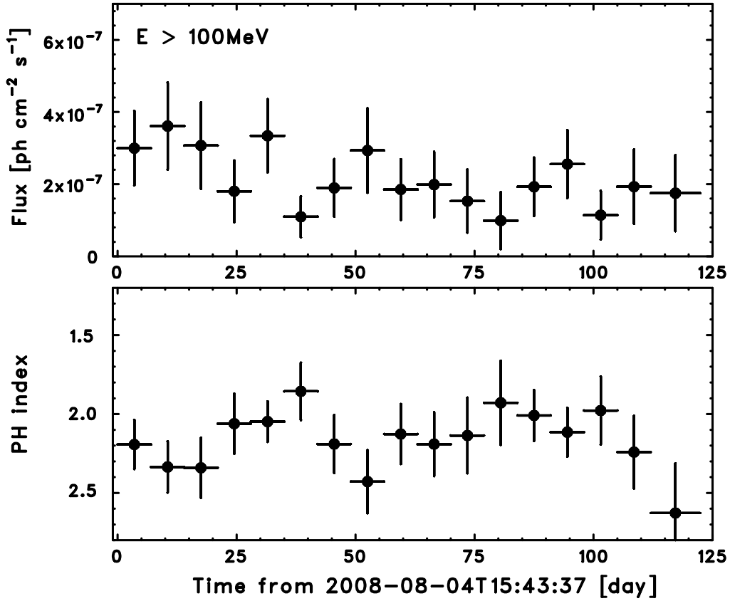
Fig. 4.— Temporal variation of \gamma -ray flux and spectral index during the 2008 August-December observation. The observation time is measured from the start of the Fermi observation, i.e., 2008 August 4 15:43:37 UT. upper panel : changes in the E > 100 MeV fluxes (calculated from an extrapolation of E > 200 MeV spectrum). lower panel : changes in the power-law photon index. Background diffuse emission (both Galactic and extra-galactic) is fixed at the best-fit parameters determined from an average spectral fitting as given in the text, and only statistical errors are shown.
