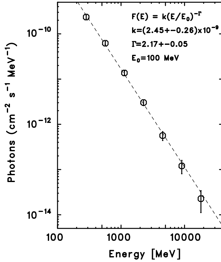
Fig. 3.— LAT spectrum of NGC 1275 from 200 MeV to 25 GeV (open circles). A dashed line (parameters given in the upper right of the figure) shows the best-fit power-law function determined from the GTLIKE as given in the text.
