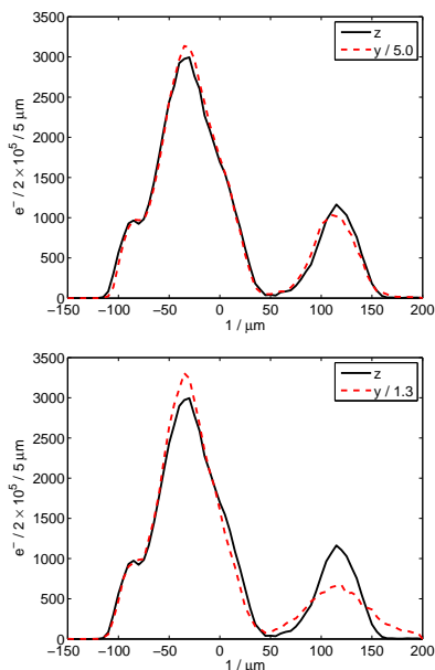
Figure 2: Final distributions of z (solid black line) and y (dashed red line) at screen downstream of X-band TCAVs (top) and S-band TCAVs (bottom) for a realistic FACET two-bunch beam simulated in Elegant [13]. Beam travels to the left.
