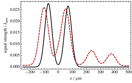
Figure 1: Calculated response of an optimized electro-optic system to a FACET-like two-bunch beam. The solid black line shows the THz field of the beam as seen by the laser pulse while traversing the crystal. The height of the THz field has been arbitrarily scaled. The dashed red line shows the final signal extracted using the balanced detection technique given as a fraction of the laser intensity incident on the EO crystal. The two right-most peaks are the reflected signal. Beam travels to the left.
