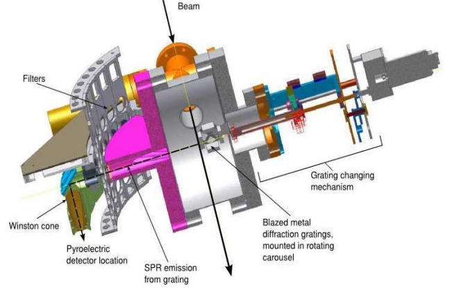
Fig. 1: Layout of the Smith-Purcell vacuum chamber
