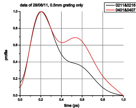
Fig. 3: Preliminary profile reconstruction of a FACET beam from the coherent SPR spectra detected in Fig. 2.
