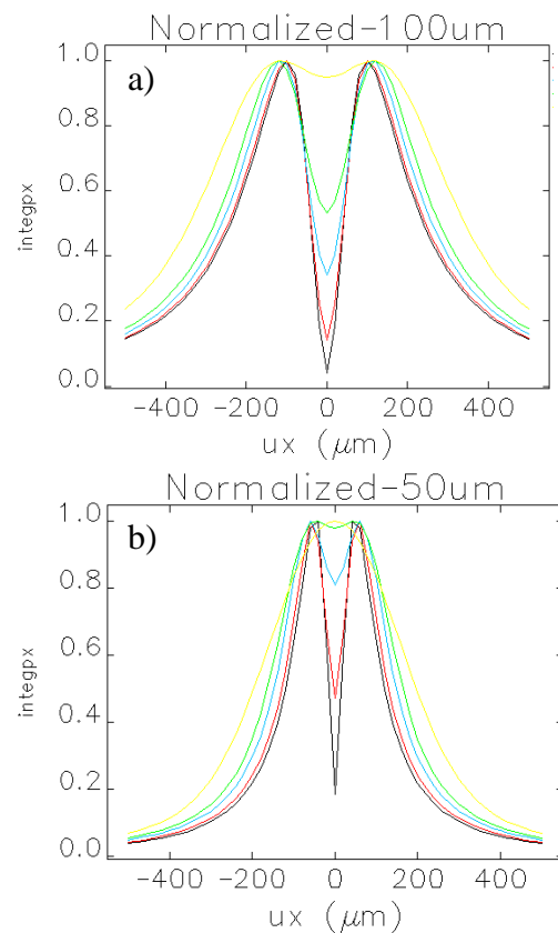
Figure 5: Numerical simulations of the ODR horizontally polarized component changes with horizontal beam size for two different impact parameters a) 100 \mu\text{m} and b) 50 \mu\text{m} . The input horizontal sizes are 10, 20, 35, 50, and 100 \mu\text{m} with the corresponding ODR profile curves in black, red, blue, green, and yellow, respectively. The vertical beam size was fixed at 10 \mu\text{m} , and the wavelength was 0.8 \mu\text{m} .
