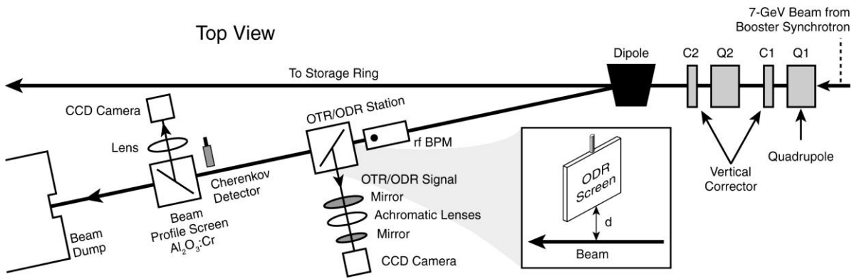
Figure. 2: Schematic of the OTR/ODR imaging station on the APS transport line. A beam of 7 GeV energy was extracted from the booster synchrotron with \sim 3 nC in a single micropulse. (From ref. 6).
