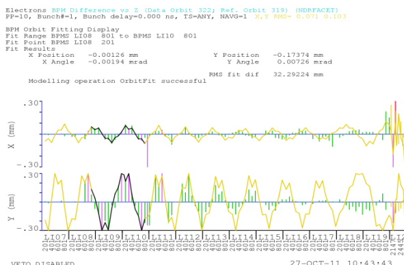
Figure 1: Orbit oscillation (green) die out near Li13 to Li15, the extrapolation (yellow) of the fit (black) shows the expected behaviour.
