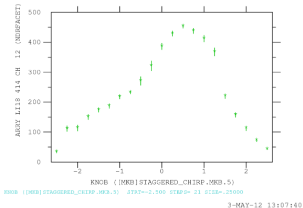
Figure 7: Peak current signal versus Linac phase indicating the right chirp for the best compression.
