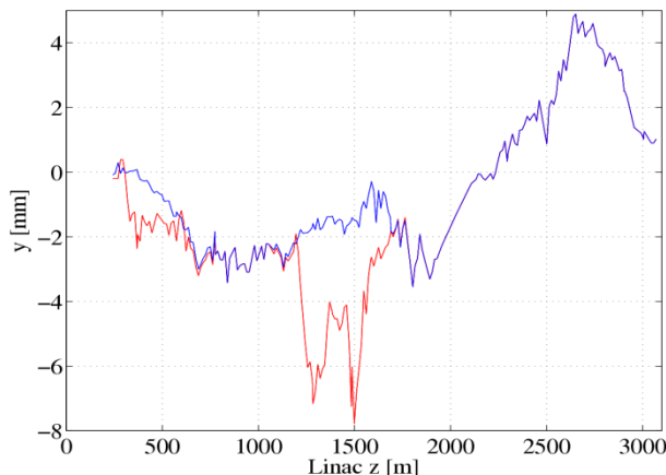
Figure 2: Vertical Linac alignment.
