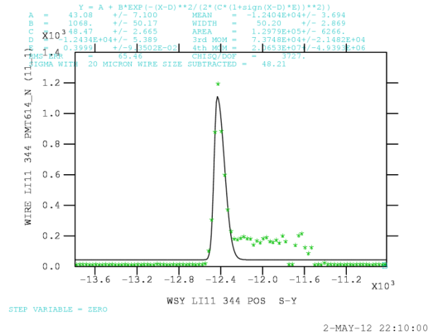
Figure 5: Wire scanner beam projection with long tail.
