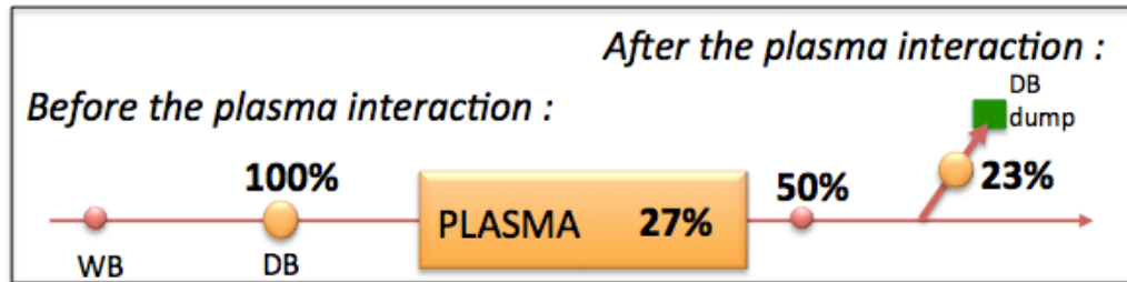
Figure 3: Power flow from an e- drive bunch (DB) to Plasma and to an e- Witness Bunch (WB), as calculated by QuickPIC.
