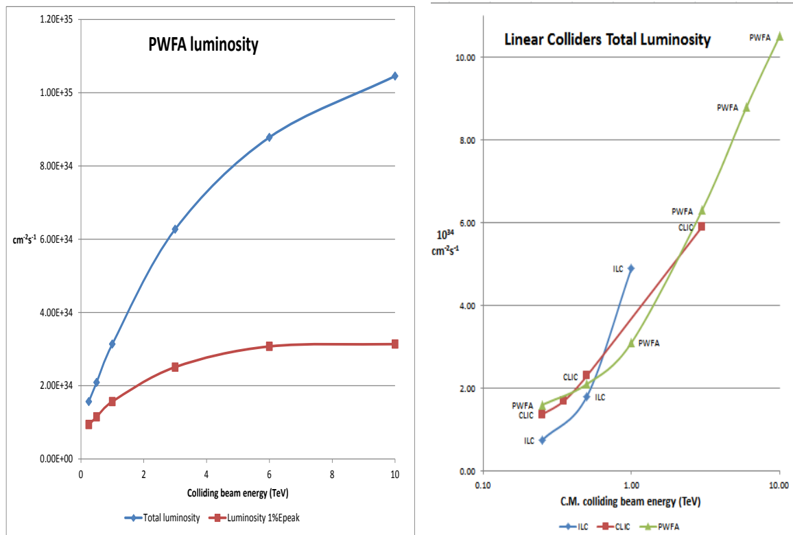
Figure 2: PWFA luminosity and comparison with other Linear Collider options
