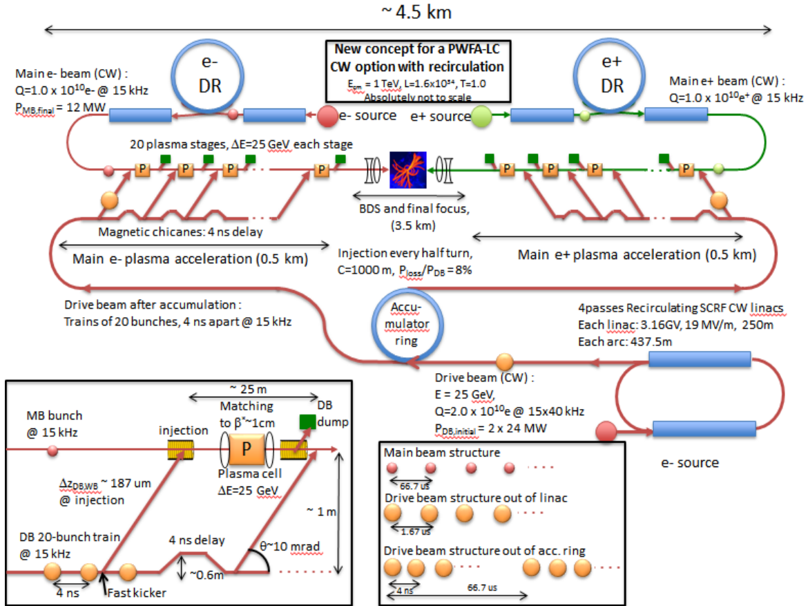
Figure 1: Layout of a 1 TeV PWFA Linear Collider
