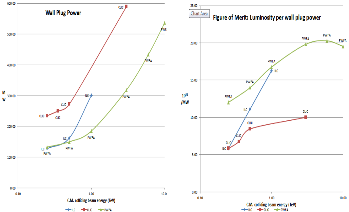
Figure 4: Wall plug power consumption and luminosity to power figure of merit in Linear Colliders
