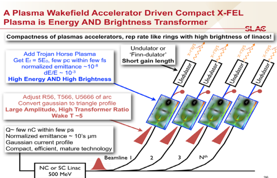
Figure 5: Layout of a PWFA based X-FEL
