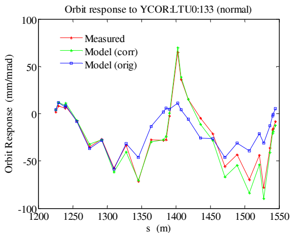
Figure 3: Fitting results (3.454 GeV).
