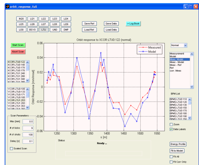
Figure 1: Orbit Response Diagnostic GUI.
