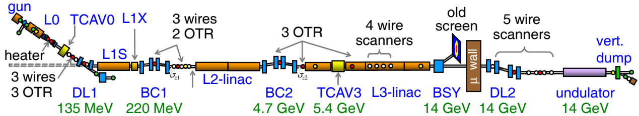
Figure 2: Layout of the LCLS accelerator.
