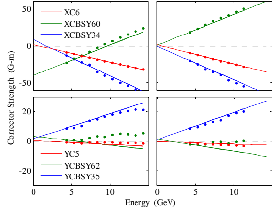
Figure 5: Beam-based static magnetic field measurement. Horizontal and vertical correctors are shown in the top and bottom panels. The panels on the left and right show the measurements before and after applying static offsets to the corrector magnets. Actual corrector strengths are dots and the solid lines are from fits to the measured orbits.
