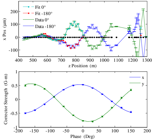
Figure 4: RF transverse orbit kick. Upper plot shows for the RF structure at 700 m the difference orbits for two phase settings w.r.t. structure off. Lower plot shows corresponding corrector strength for x & y plane vs. RF phase.
