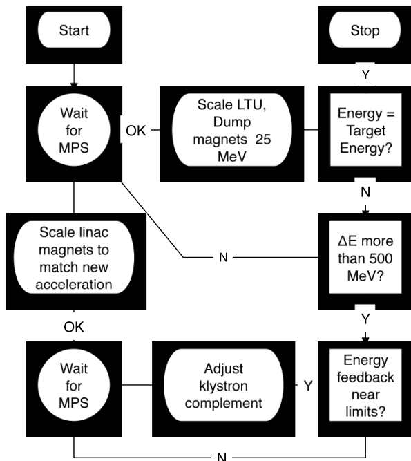
Figure 3: Process flow of the Energy Ramp GUI. The steps marked “Wait for MPS” check that the beam has not tripped off for any reason and that the operator has not pressed the pause button.
