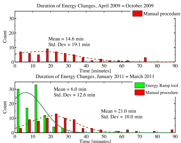
Figure 5: Energy change statistics for the Energy Ramp GUI (green) vs. the written procedure (red). Data were collected from the LCLS operations logbook and histogrammed into 5-minute bins. The Energy Ramp GUI is both faster on average and more predictable.
