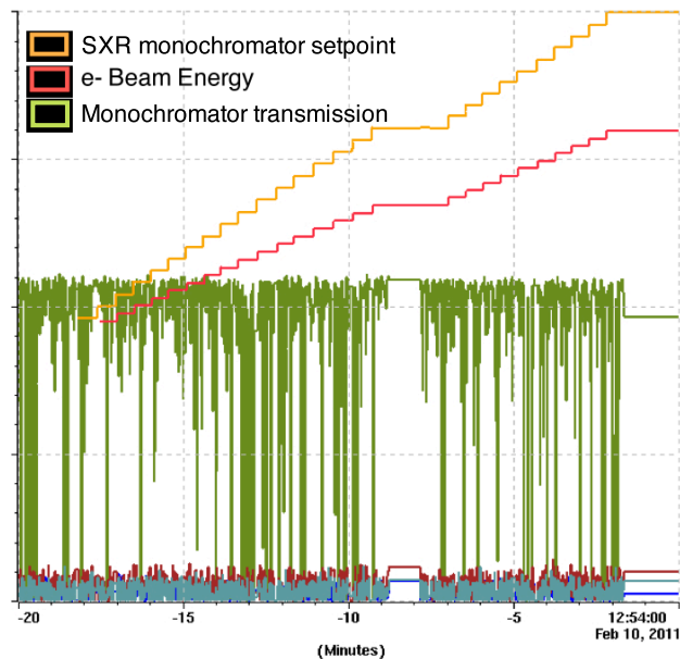
Figure 6: Controlling the electron beam energy with the SXR monochromator. As the monochromator grating (yellow) is tilted to scan from 810 to 840 eV, the Energy Ramp GUI scales the electron beam energy (red) to match.
