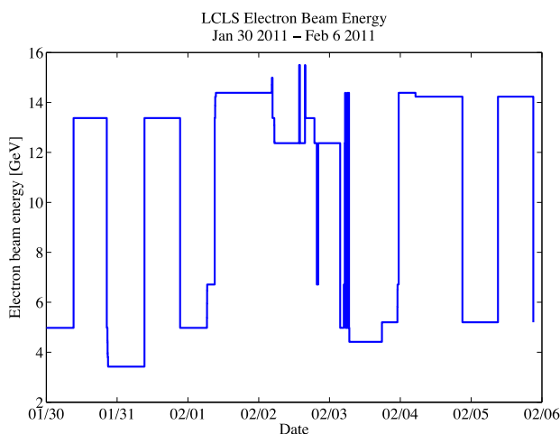
Figure 1: Electron beam energy over a typical week of user operation at LCLS, from Sunday to Sunday. Accelerator physics studies take place in the middle of the week.
