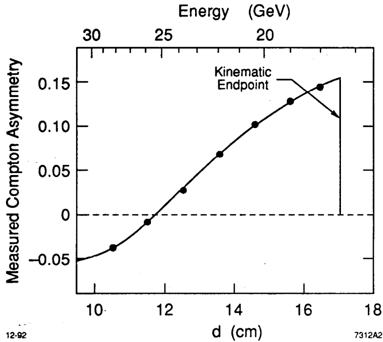
Figure 1. The average polarized Compton scattering asymmetry as measured by seven channels of the Cherenkov detector is plotted as a function of the distance ( d ) from the trajectory of the undeflected beam. The curve represents the product of the asymmetry function and a normalization factor that has been adjusted to achieve a best fit to the measurements.
