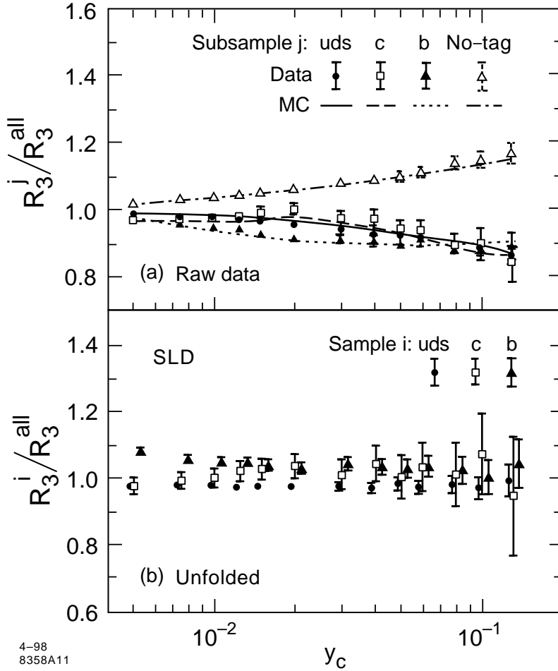
Figure 5: (a) The raw measured ratios R_3^j/R_3^{all} , 1 \leq j \leq 4 , vs. y_c for the 4 subsamples (see text); data (points with error bars), and simulation (lines joining values at the same y_c values as the data). (b) The unfolded ratios R_3^i/R_3^{all} , i = b, c, uds , vs. y_c for the 3 primary event flavor groups. Only statistical errors are shown. In (b) points corresponding to a common y_c value have been displaced horizontally for clarity.
