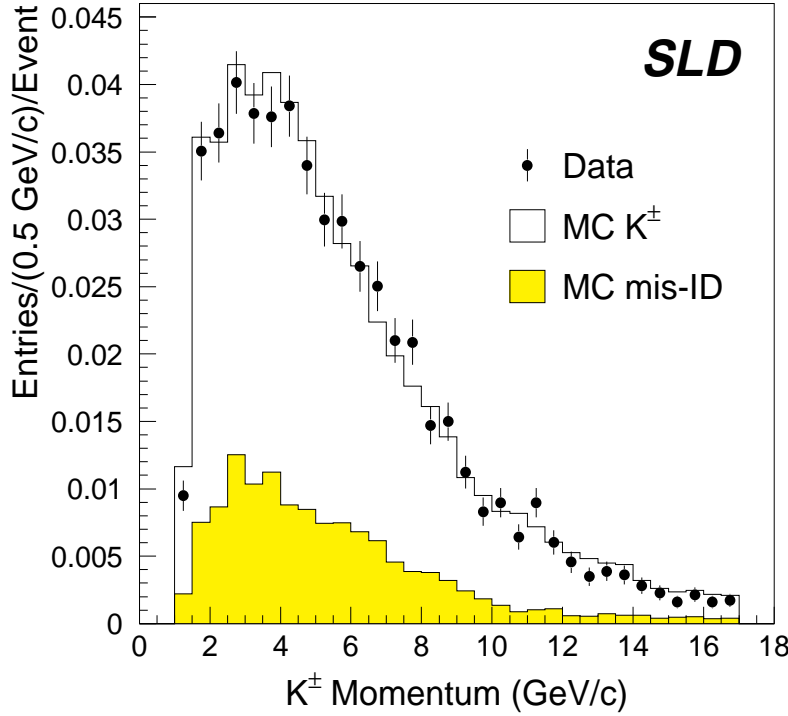
Figure 1: Momentum distribution of selected B decay K^\pm candidates.
