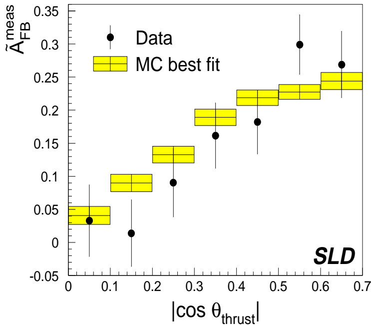
Figure 2: Measured left-right forward-backward asymmetry for b\bar{b} events as a function of thrust axis \cos\theta for background-corrected data (points). The shaded boxes correspond to the best fit MC, where the vertical size of each box spans the \pm 1\sigma MC statistical errors.
